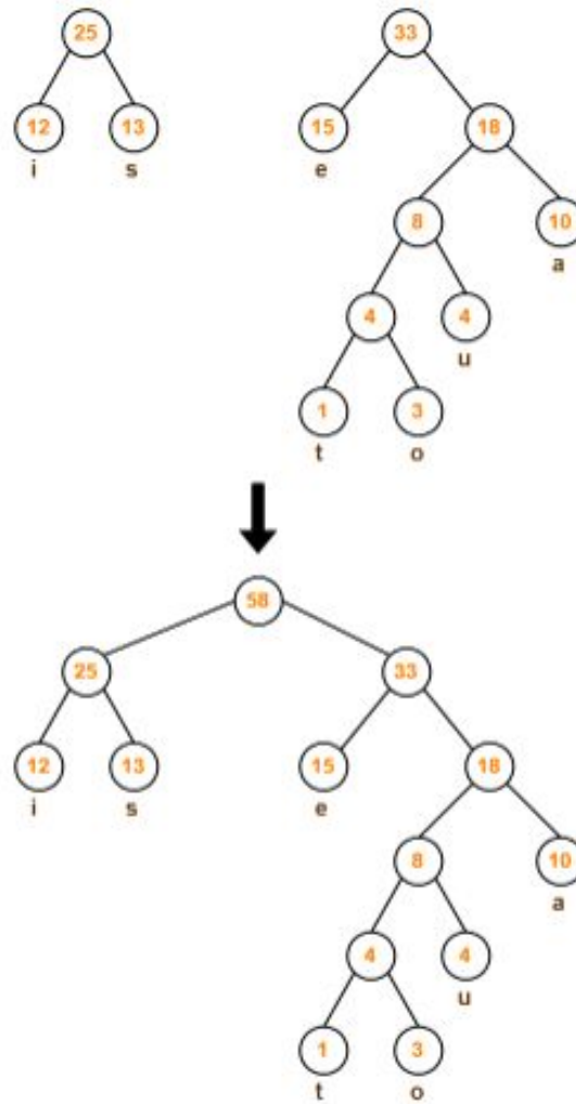
Huffman Tree
